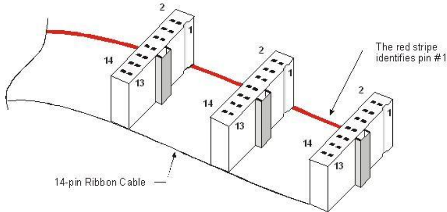
Figure 3. CDS-14-3 cable
