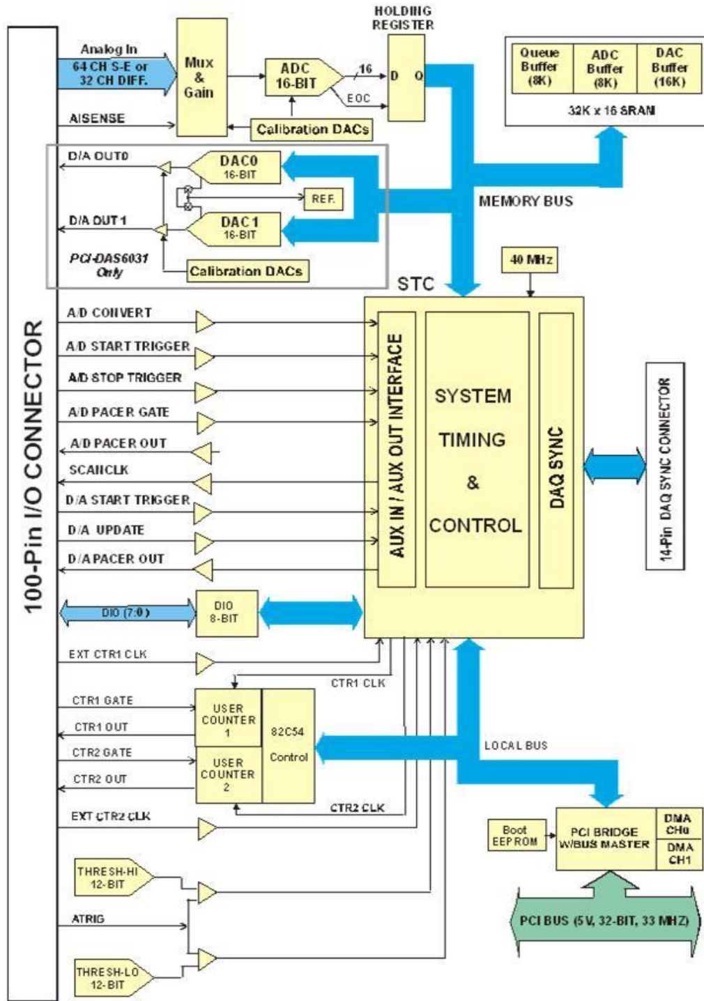
Figure 4. Functional block diagram
