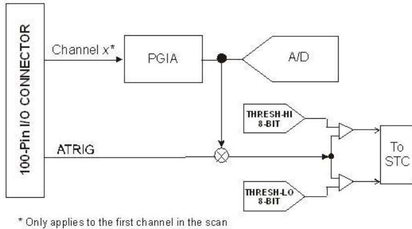
Figure 18. ATRIG circuit
