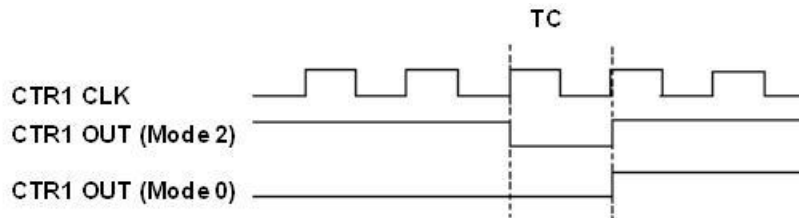
Figure 34. CTR1 OUT signal timing
