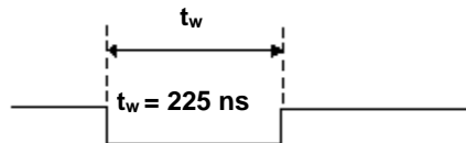
Figure 30. D/A CONVERT output signal timing
