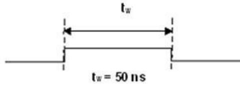
Figure 28. D/A START TRIGGER output signal timing
