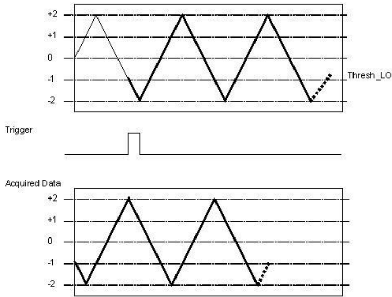
Figure 20. Trigger Negative Slope
