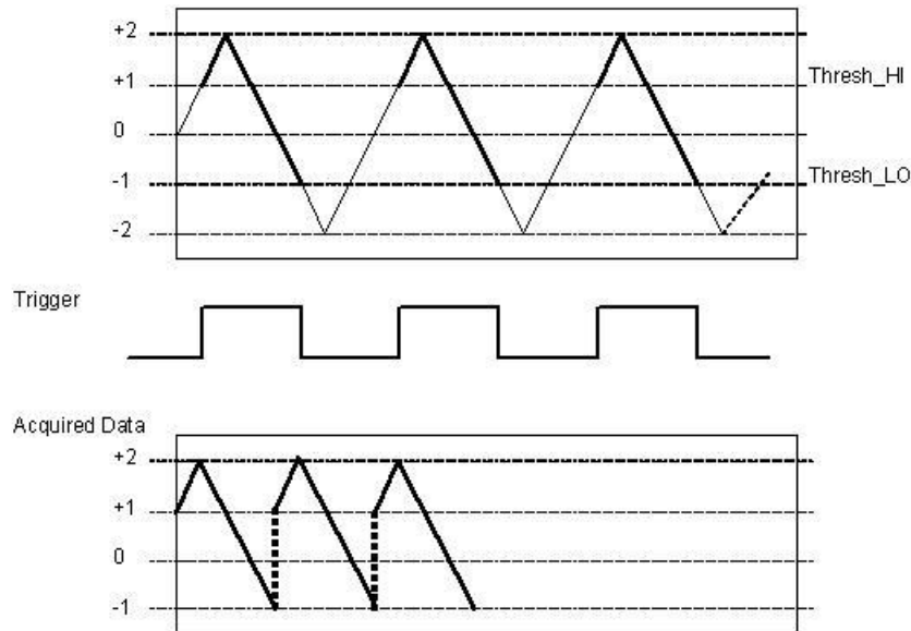
Figure 23. Gate Negative Hysteresis
