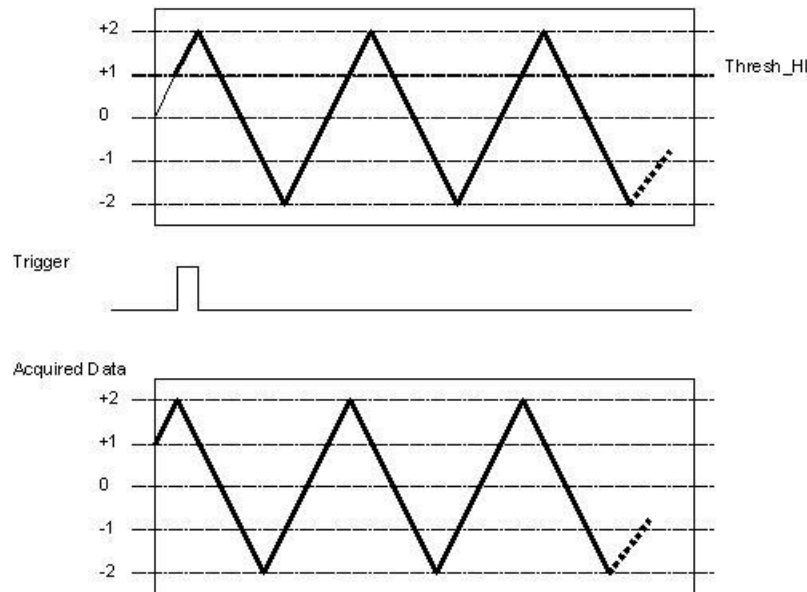
Figure 19. Trigger Positive Slope
