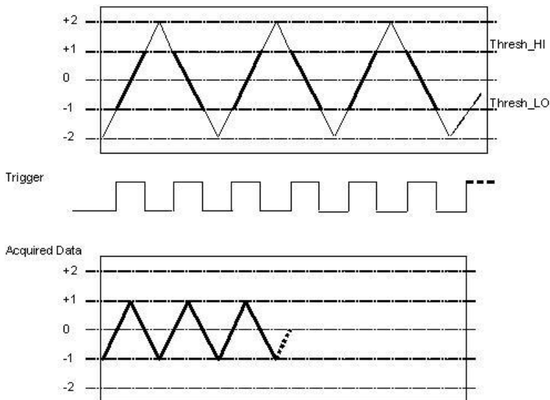
Figure 25. Gate Inside Window
