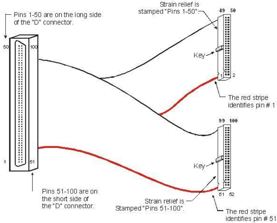
Figure 1. C100HD50-x cable
