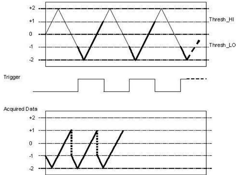
Figure 24. Gate Positive Hysteresis
