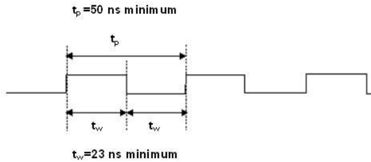
Figure 31. D/A EXTERNAL TIME BASE signal timing
