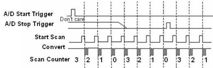
Figure 10. Pre-triggered data acquisition example
