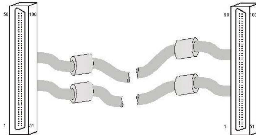
Figure 2. C100MMS-x cable
