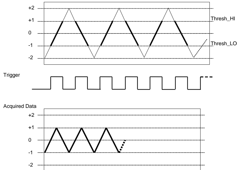
Figure 25. Gate Inside Window
