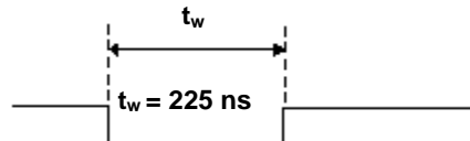
Figure 30. D/A CONVERT output signal timing
