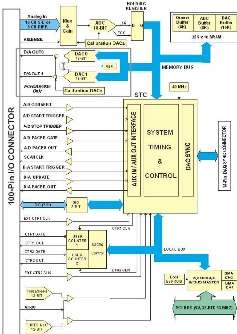
Figure 4. Block diagram – PCI-DAS6030/32
