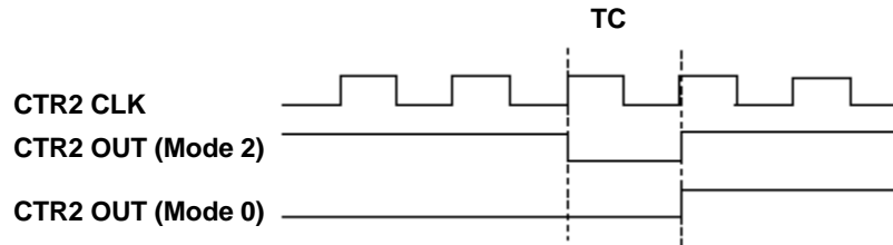
Figure 37. CTR2 OUT signal timing
