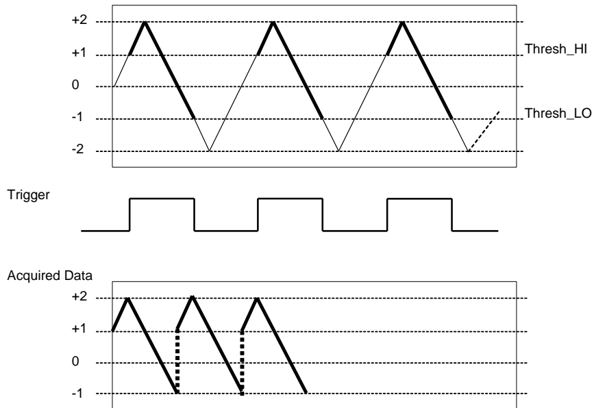
Figure 23. Gate Negative Hysteresis
