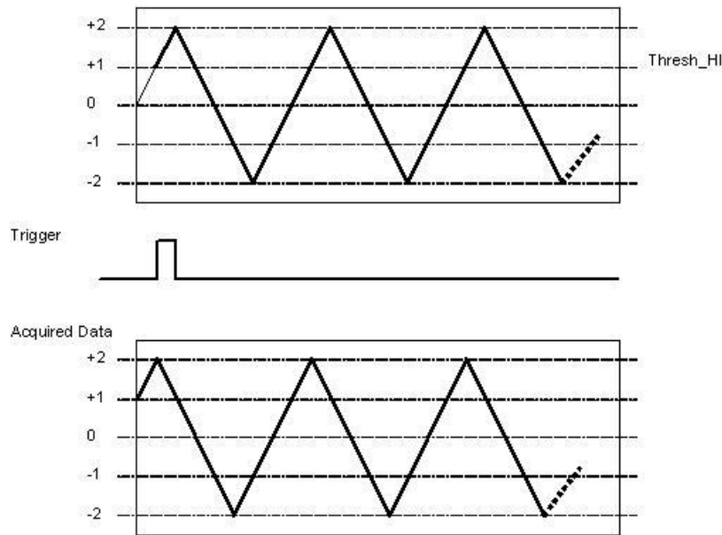
Figure 19. Trigger Positive Slope
