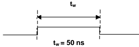
Figure 28. D/A START TRIGGER output signal timing
