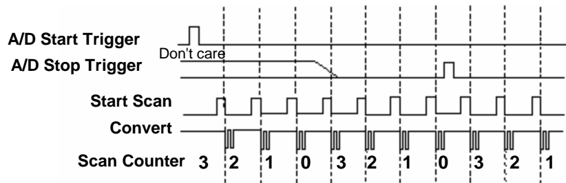
Figure 9. Pre-triggered data acquisition example
