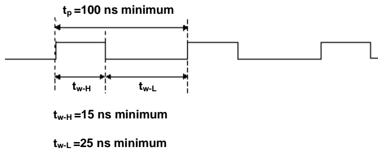
Figure 35. CTR2 CLK signal timing
