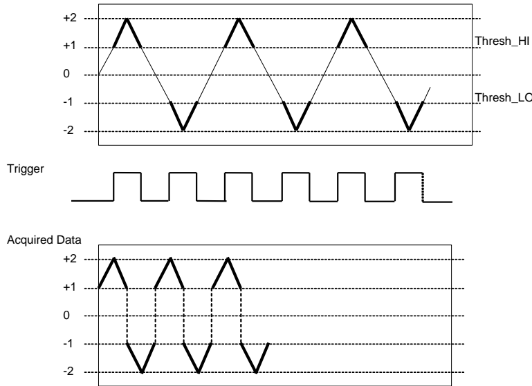
Figure 26. Gate Outside Window
