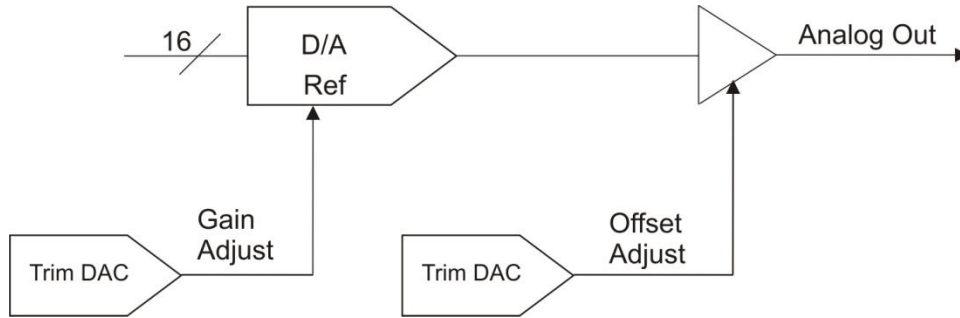
Figure 39. Analog output calibration – basic elements
