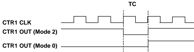
Figure 34. CTR1 OUT signal timing
