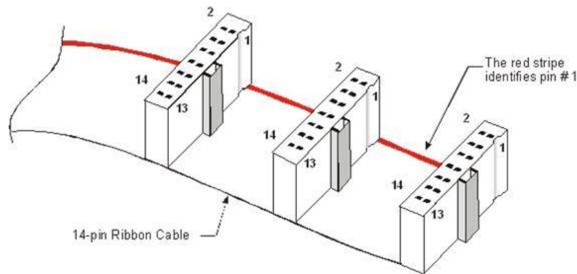
Figure 3. CDS-14-3 cable
