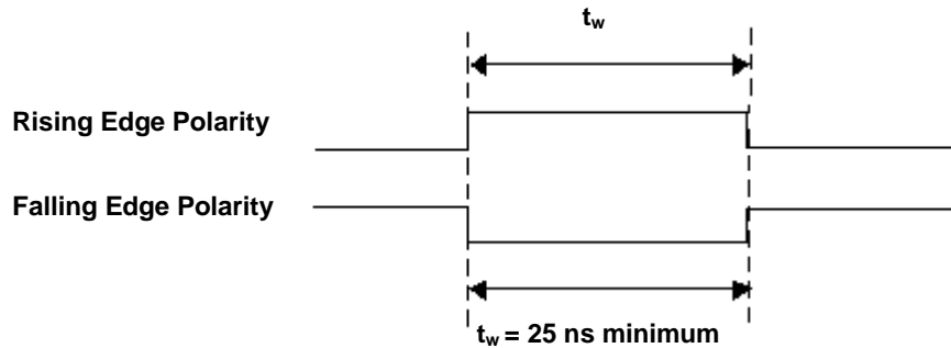
Figure 33. CTR1 GATE signal timing
