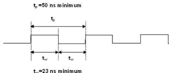
Figure 31. D/A EXTERNAL TIME BASE signal timing
