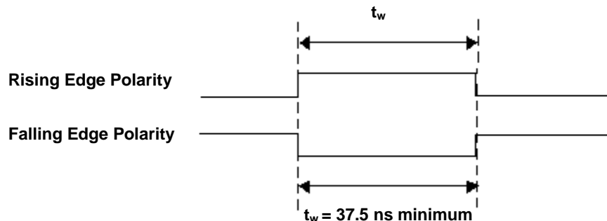
Figure 27. D/A START TRIGGER input signal timing
