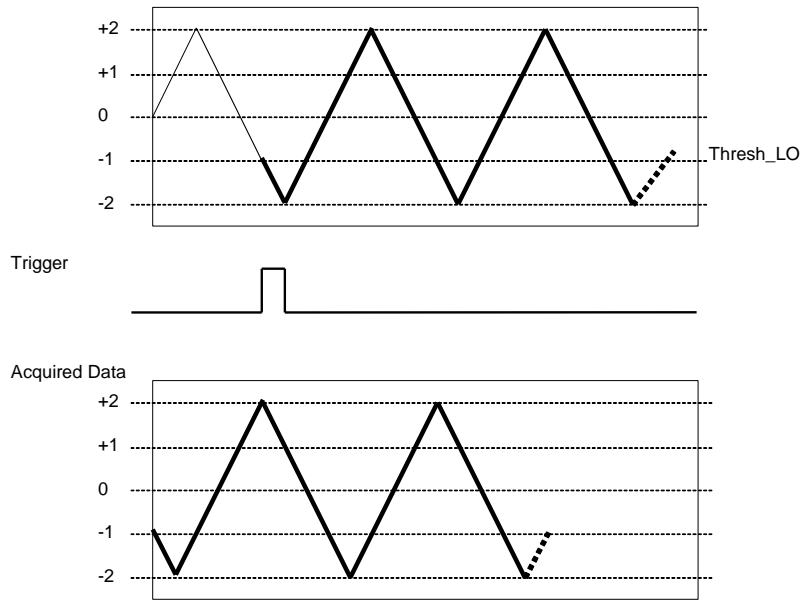
Figure 20. Trigger Negative Slope
