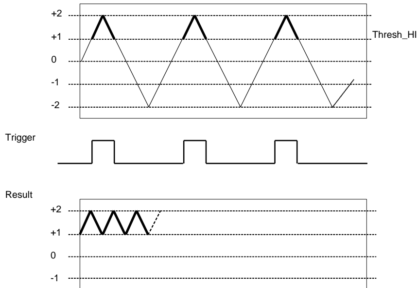
Figure 21. Gate Above
