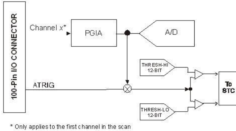
Figure 18. ATRIG Circuit
