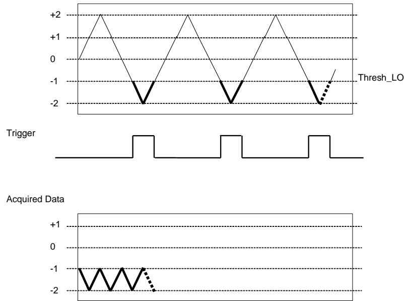
Figure 22. Gate Below
