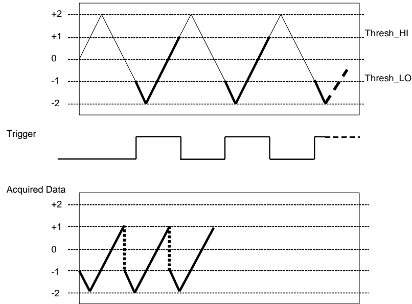
Figure 24. Gate Positive Hysteresis
