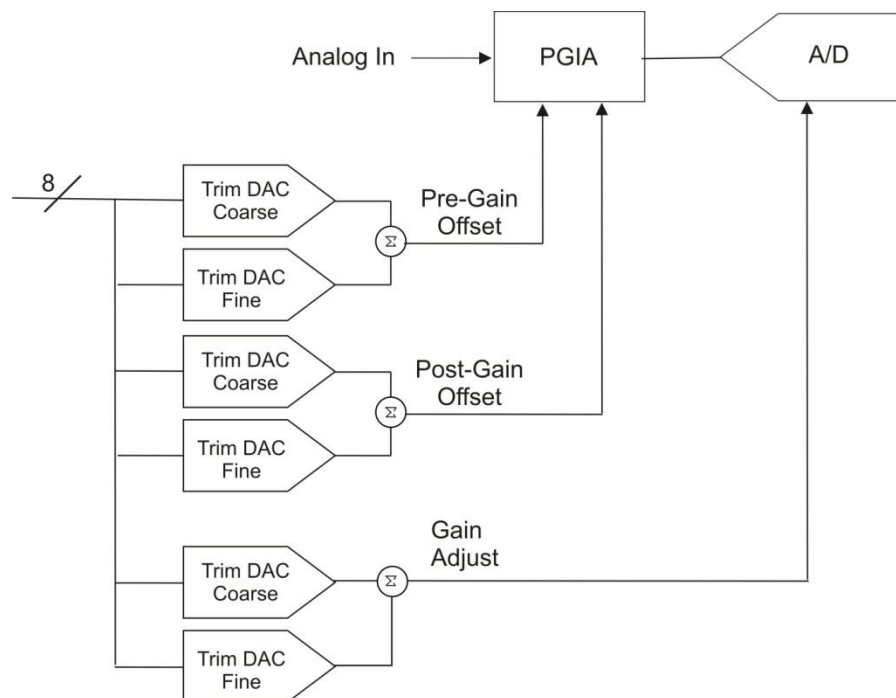
Figure 38. Analog input calibration - basic elements
