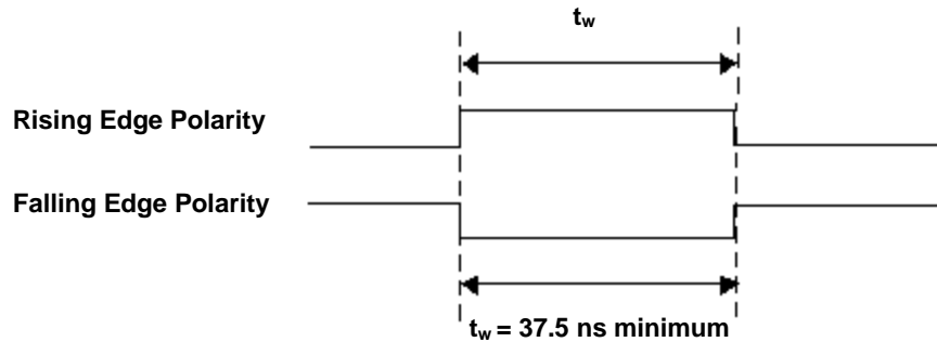
Figure 29. D/A CONVERT input signal timing
