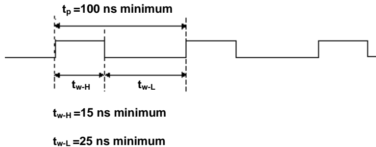
Figure 32. CTR1 CLK signal timing
