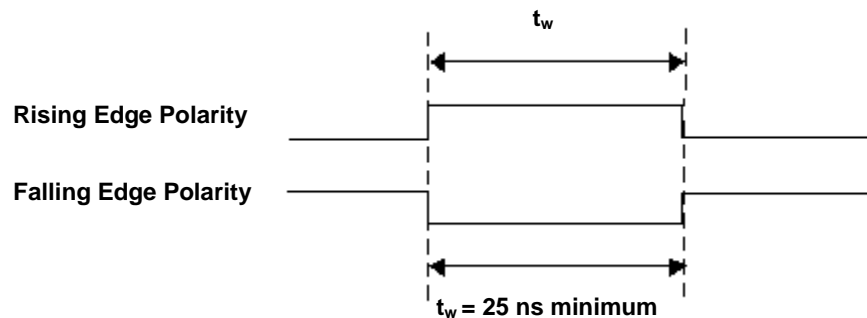
Figure 36. CTR2 GATE signal timing
