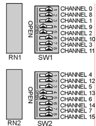
DBK1 Resistor Configuration
