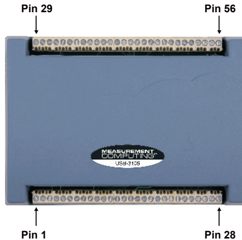
Figure 4. USB-3105 screw terminal pinout numbering
