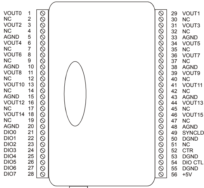
Figure 5. USB-3105 signal pinout
