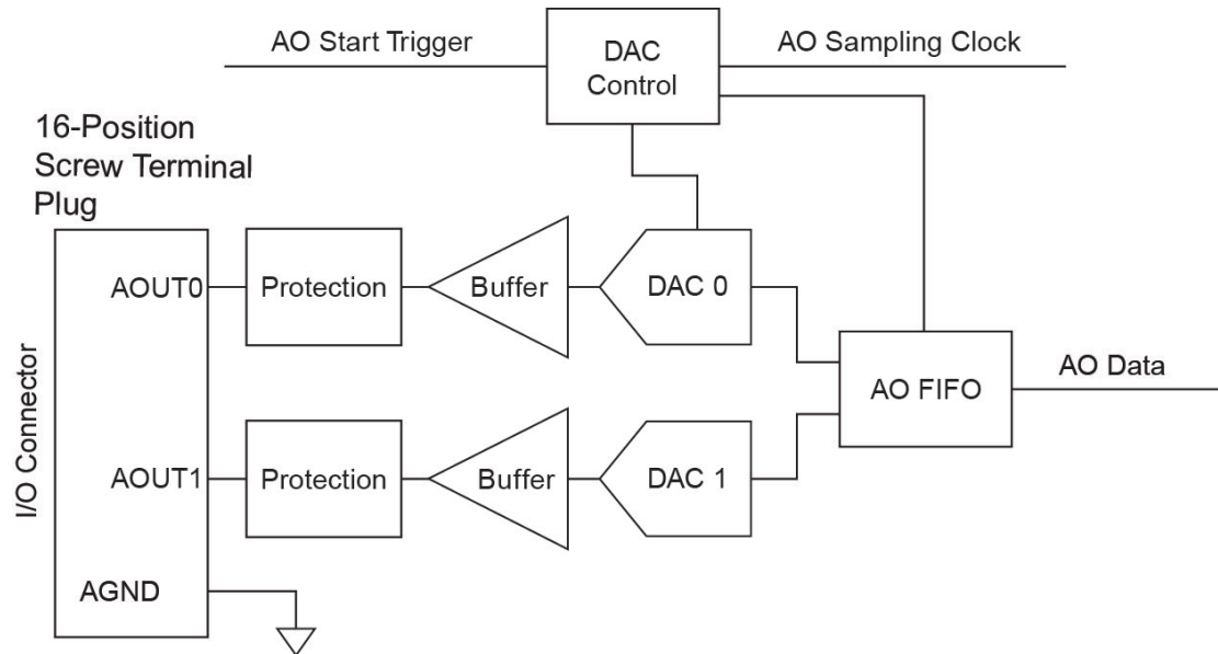
Figure 8. USB-231 analog output circuitry
