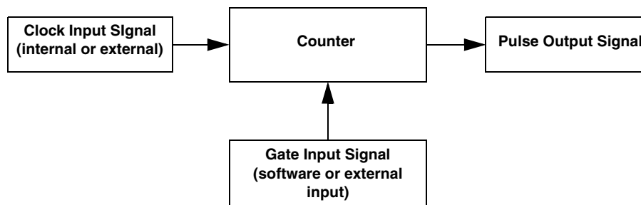
Figure 9: Counter/Timer Channel
