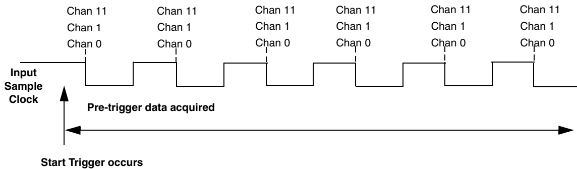
Figure 8: Continuous Sampling Mode on the DT7816 Module
