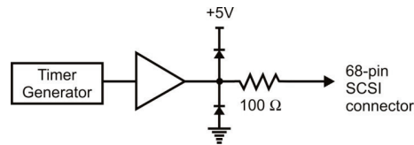
Figure 16. Typical PCI-2513 timer channel
