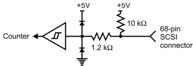
Figure 5. Typical PCI-2513 counter channel
