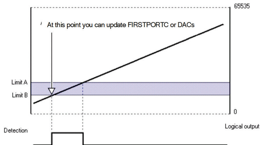
Figure 21. Channel 1 in totalizing counter mode, inside the window setpoint
