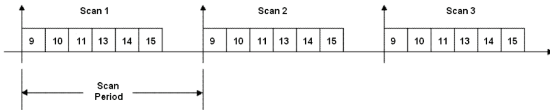
Figure 14. PCI-2513 acquisition of six readings per scan
