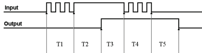
Figure 7. Debounce module – trigger after stable mode
