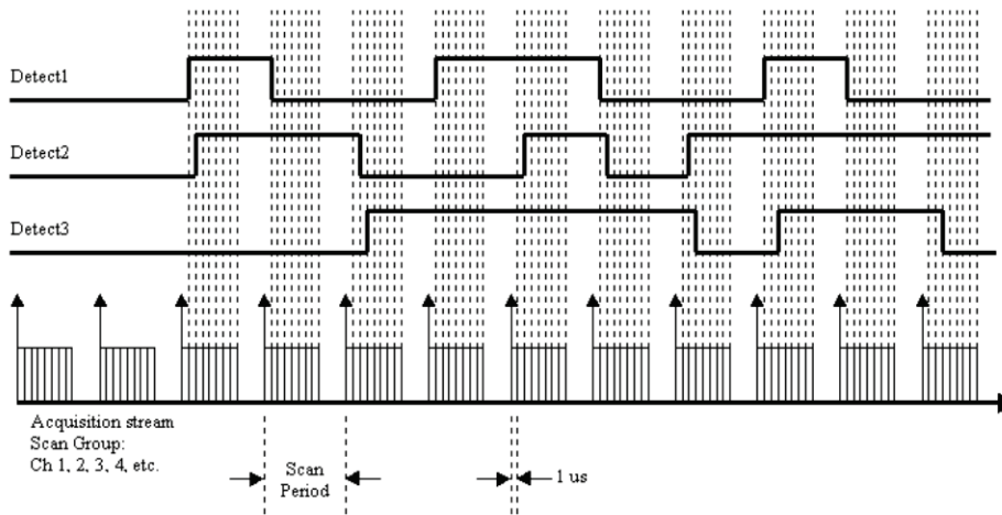
Figure 17. Example diagram of detection signals for channels 1, 2, and 3
