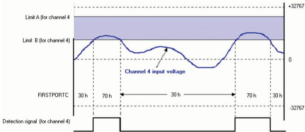
Figure 18. Analog inputs with setpoints update on True and False
