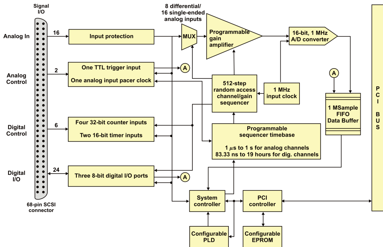
Figure 3. PCI-2513 functional block diagram
