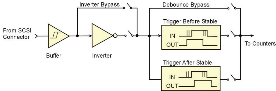
Figure 6. Debounce model block diagram
