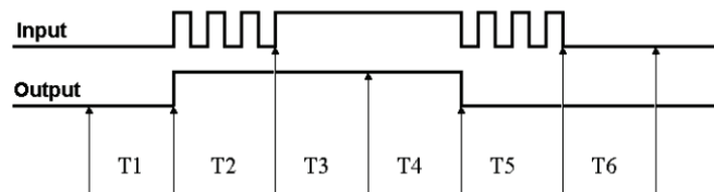
Figure 8. Debounce module – Trigger before stable mode
