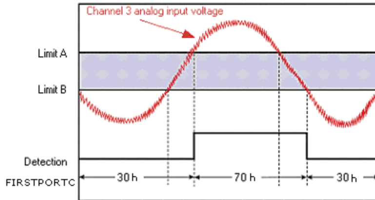
Figure 20. Channel 3 in hysteresis mode
