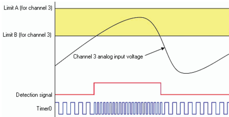
Figure 19. Timer output update on True and False
