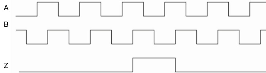
Figure 12. Representation of quadrature encoder outputs: A, B, and Z
