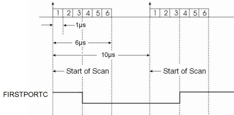
Figure 22. Example of FIRSTPORTC latency
