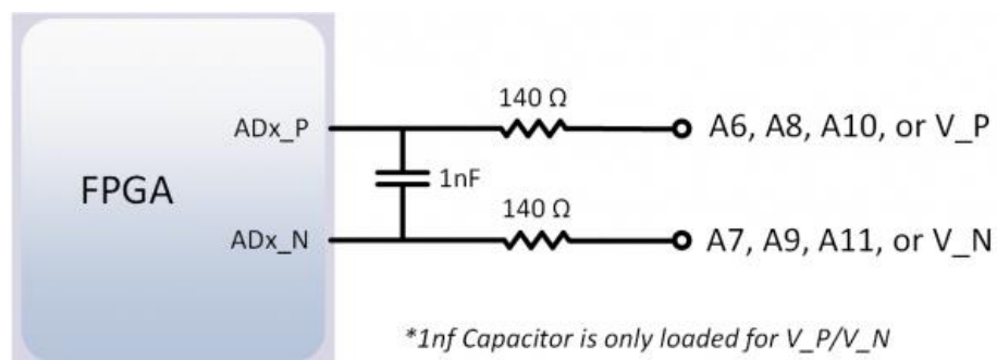
Figure 13.2.2. Differential Analog Inputs.
