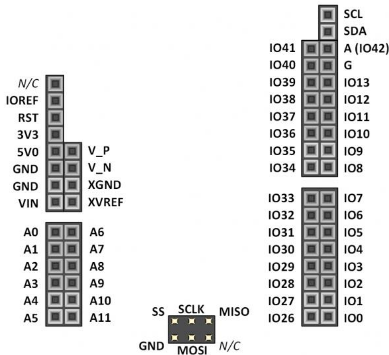
Figure 13.1. Shield connector pin diagram.
