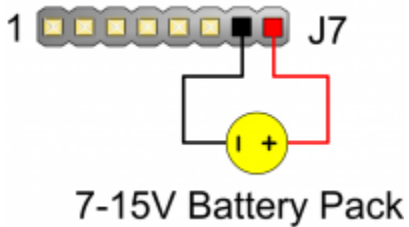
Figure 5.2. Arty S7 Battery Pack Connection.
