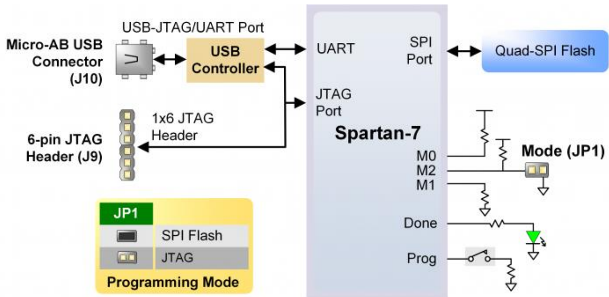
Figure 6.1. Arty S7 FPGA Configuration.
