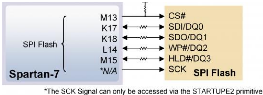
Figure 8.1. Arty S7 SPI flash.
