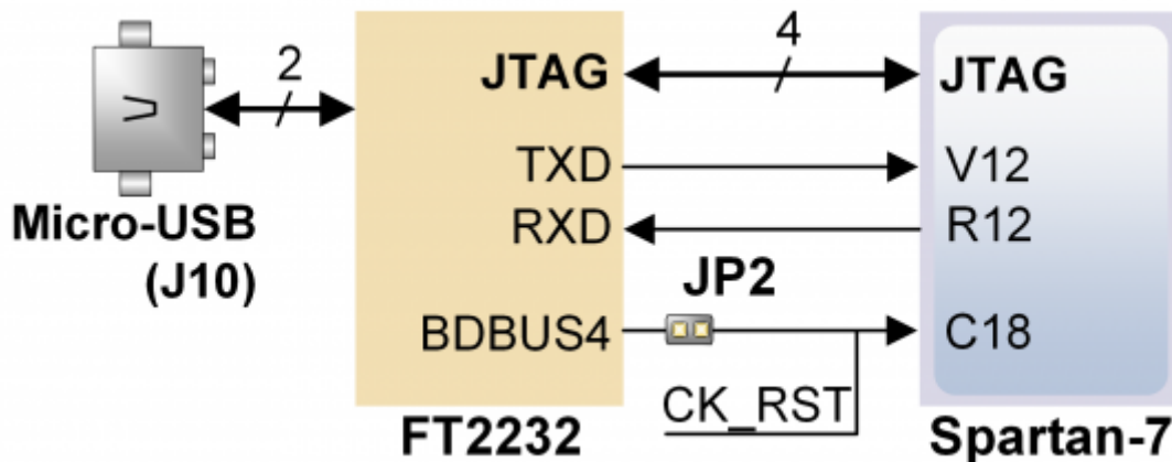
Figure 10.1. UART Connections.
