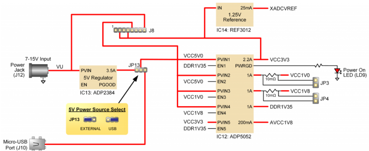
Figure 5.1. Arty S7 Power Circuit.
