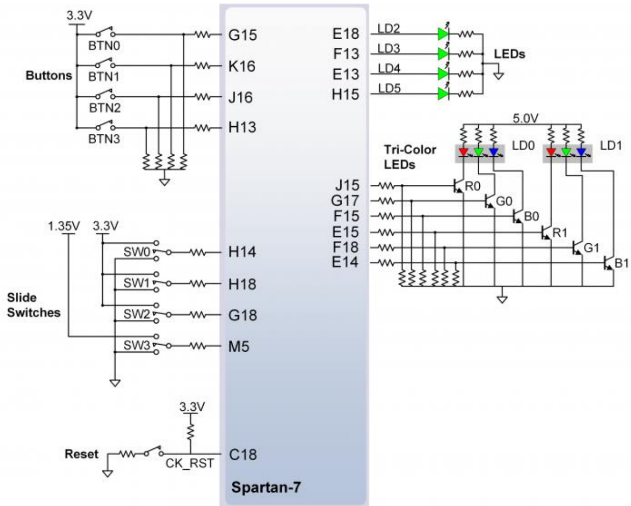
Figure 11.1. Arty S7 GPIO.
