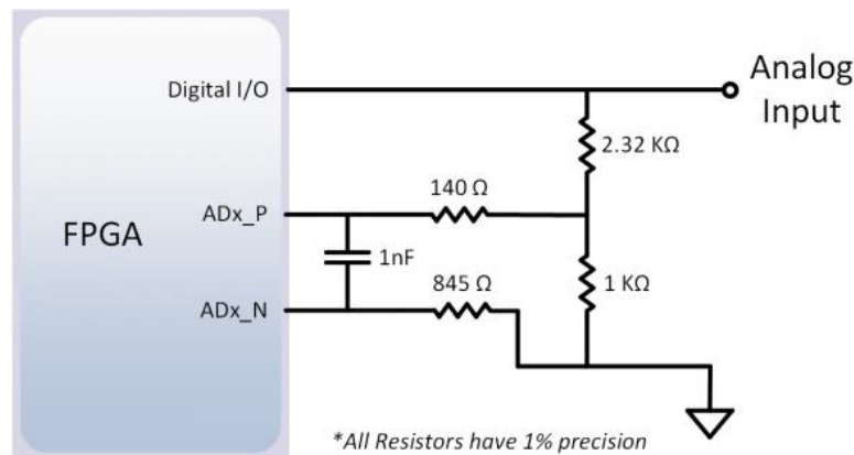
Figure 13.2.1. Single-Ended Analog Inputs.
