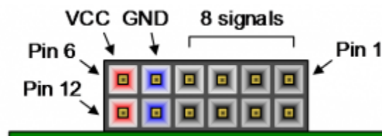
Figure 12.1. Pmod connector.
