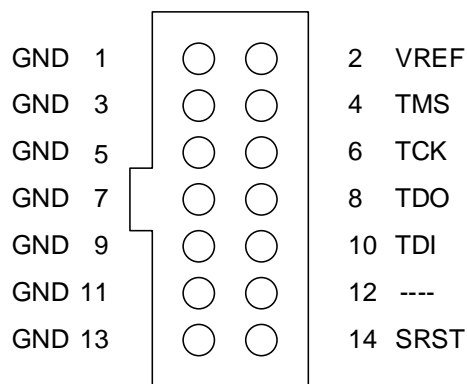
Figure 3. JTAG-HS3 pinout.
