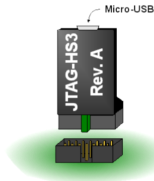
Figure 2. Xilinx JTAG header. Dual row, 2mm, 14 pin.
