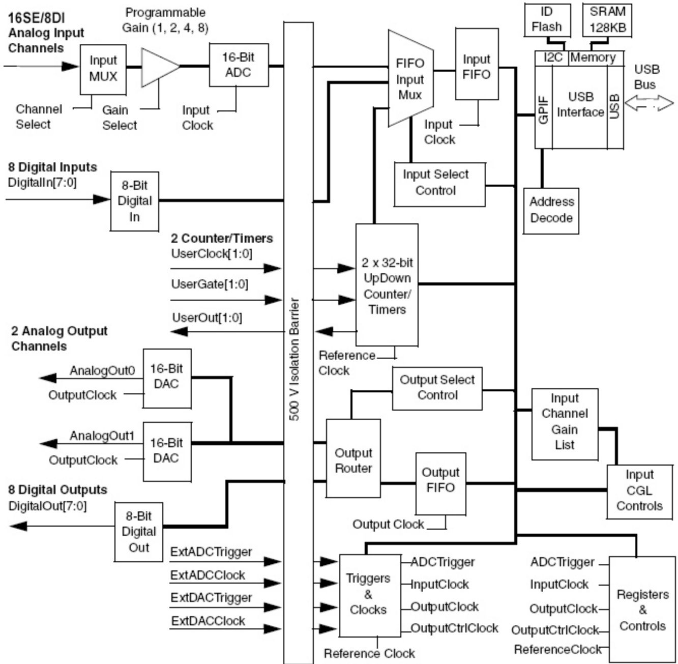
The in-depth DT9818 block diagram shows all functions and controls.
