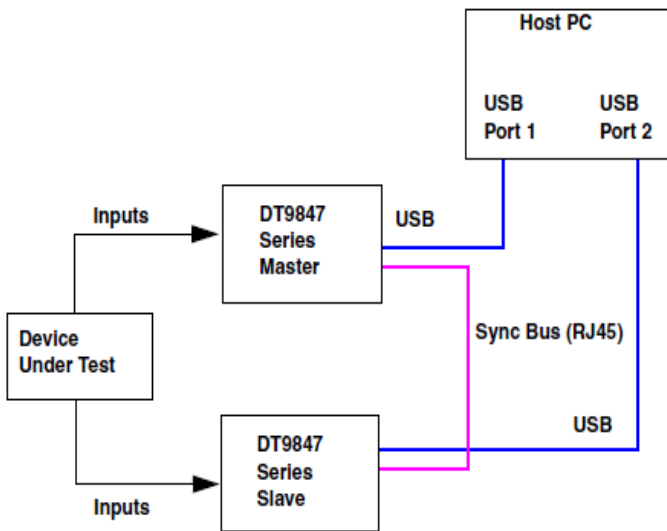
Synchronizing two DT9847 Series modules by daisy chaining the RJ45 connectors (shown using external trigger)
