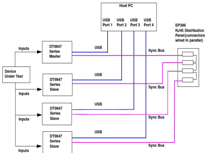
Synchronizing four DT9847 Series modules by using the EP386 RJ-45 Distribution Panel.
