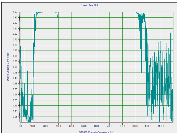
Coherence Reference Response
