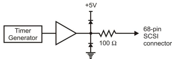
Figure 23. Typical USB-2523 timer channel
