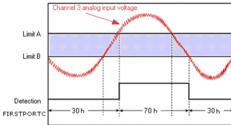
Figure 27. Channel 3 in hysteresis mode
