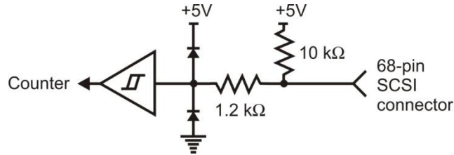
Figure 12. Typical USB-2523 counter channel
