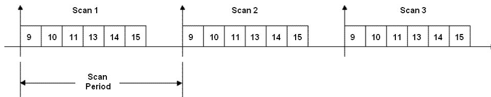
Figure 21. USB-2523 acquisition of six readings per scan
