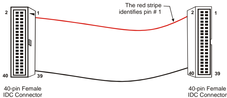
Figure 5. C40FF- x cable
