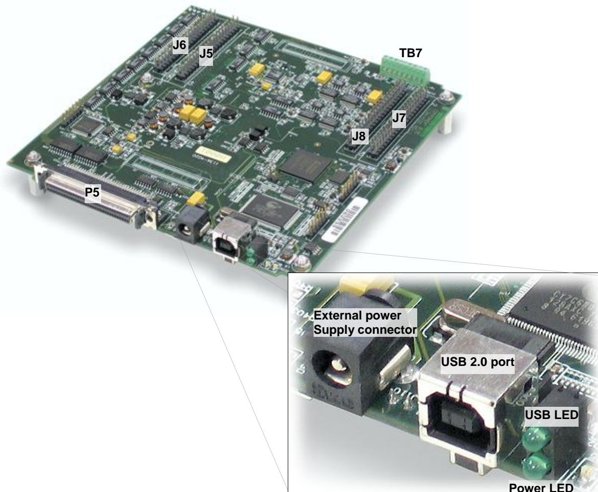
Figure 6. USB-2523 components
