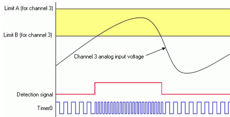
Figure 26. Timer output update on True and False
