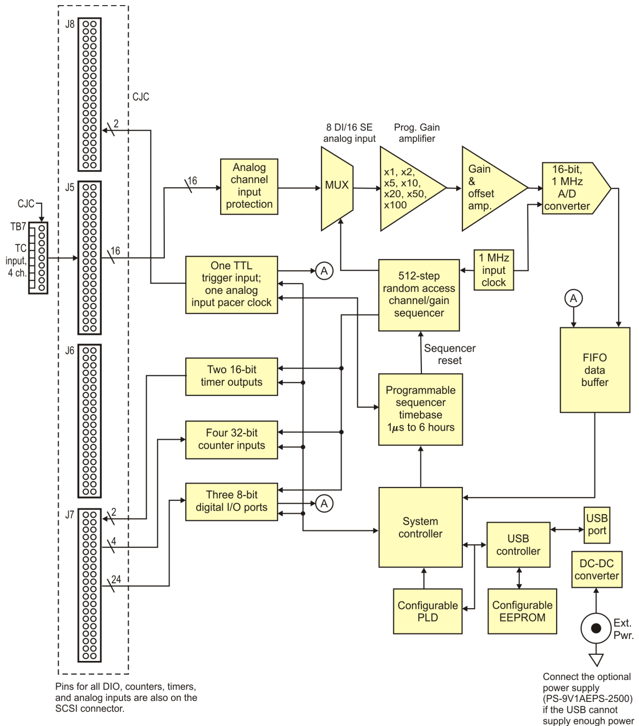
Figure 7. USB-2523 functional block diagram
