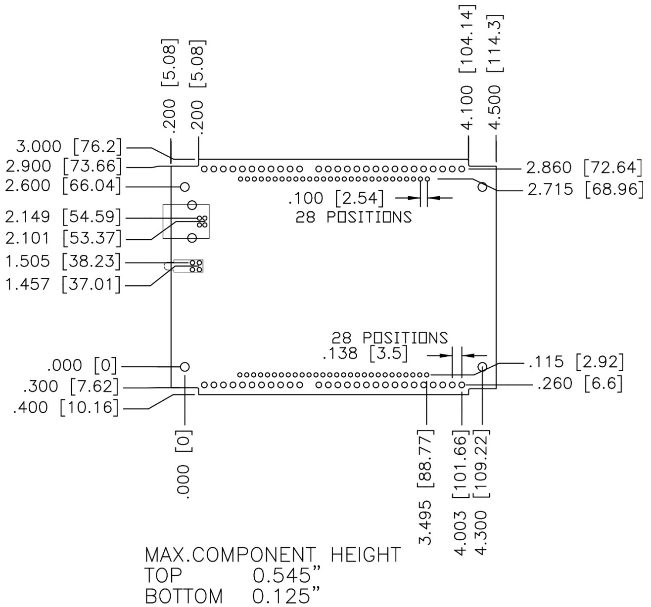
Figure 9. USB-1808X-OEM circuit board dimensions
