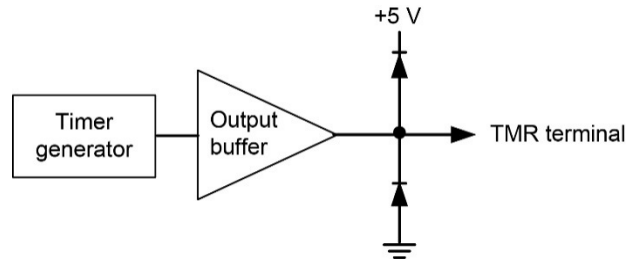
Figure 6. USB-1808X-OEM PWM timer channel
