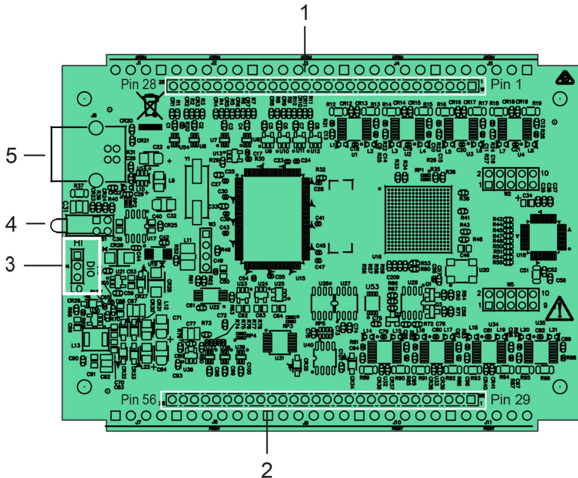
Figure 2. USB-1808X-OEM components
