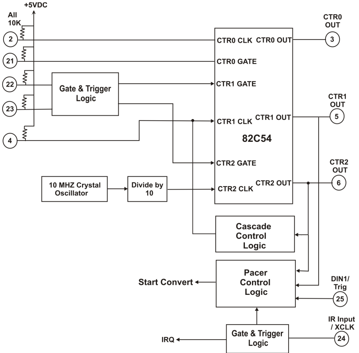
Figure 8. Pacer/counter/timer block diagram
