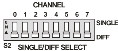
Figure 2. Input configuration jumpers
