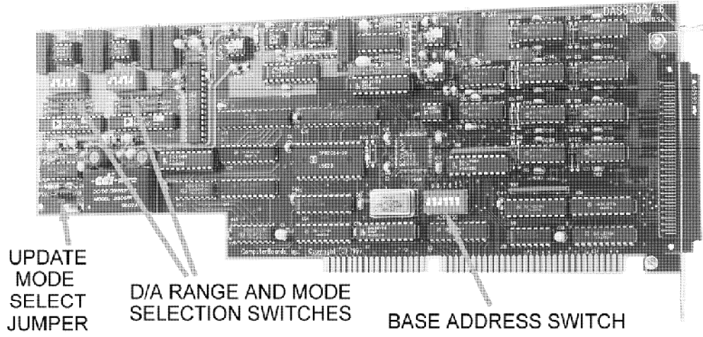
Figure 3-7. CIO-DAS6402/16 Base Address, D/A Range & Mode Switches Location
