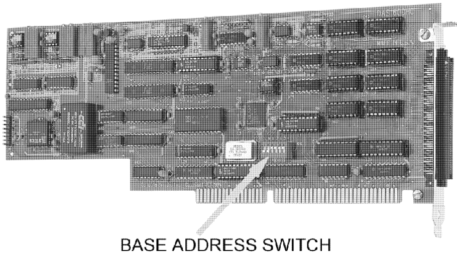
Figure 3-6. CIO-DAS6402/12 Base Address Switches Location
