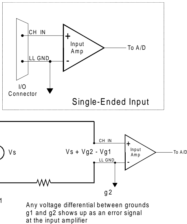
Single-ended input with Common Mode Voltage
