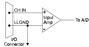
SINGLE-ENDED INPUT
